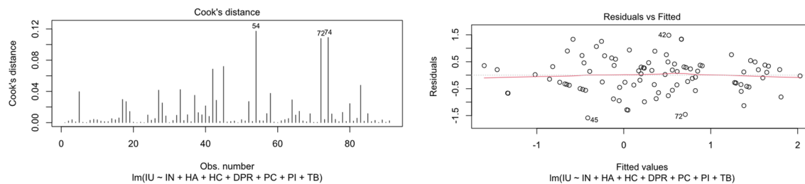
Figure 3: (L) Analysis of influential points: Cook's distance; (R) Homoscedasticity check: Residuals vs Fitted values
