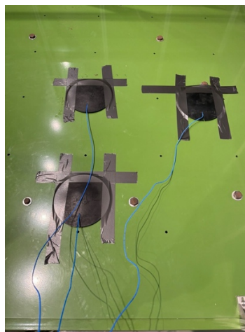
Figure 1: The experiment involved installing acceleration sensors at three distinct positions on the platform. Right and rear sensors were positioned 50 cm away from the central one.
